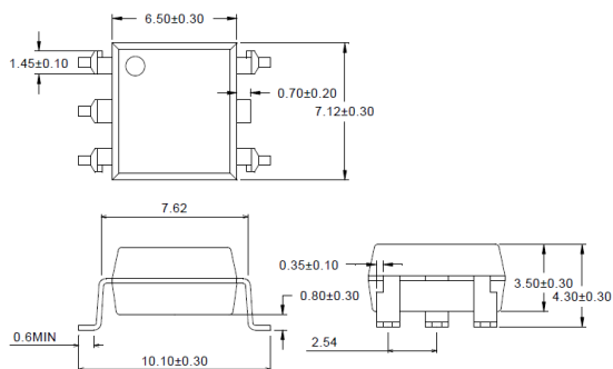
S Type
