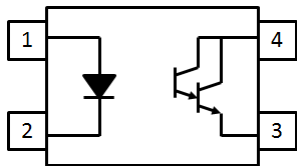
Darlington Transistor Output Type
