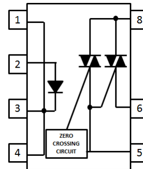
Zero Cross Type
