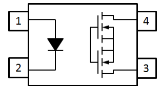
Form-A contact
