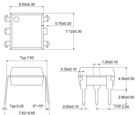
DIP Type
